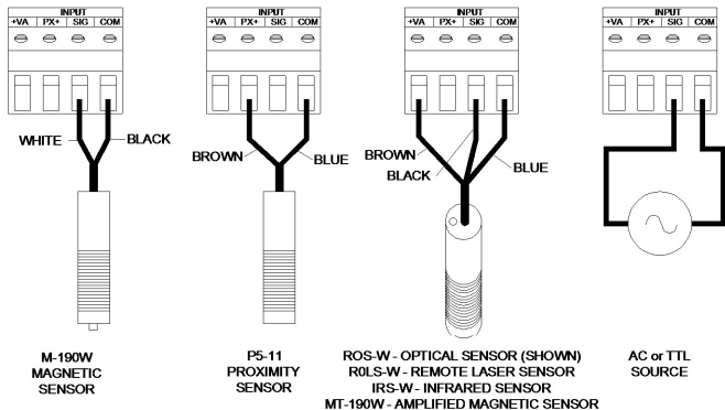
Figure 3 Sensor Connections
